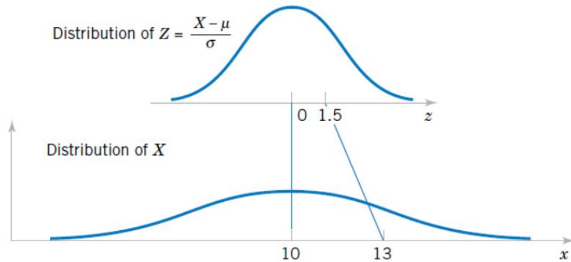
Figure 4-15 Standardizing a normal random variable.
